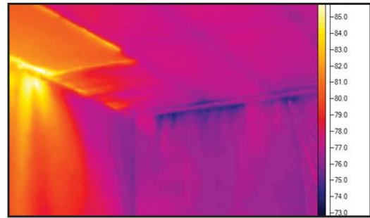
Image 9. Hot and cold thermal patterns appear next to each other in this photo.
